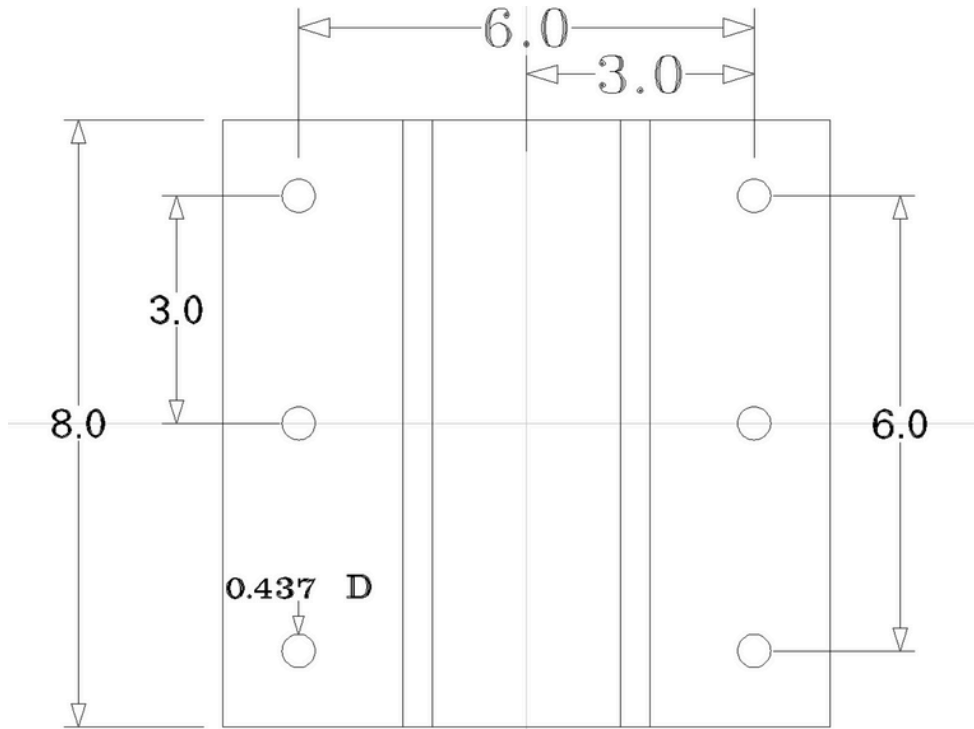
Mounting Base Plate
