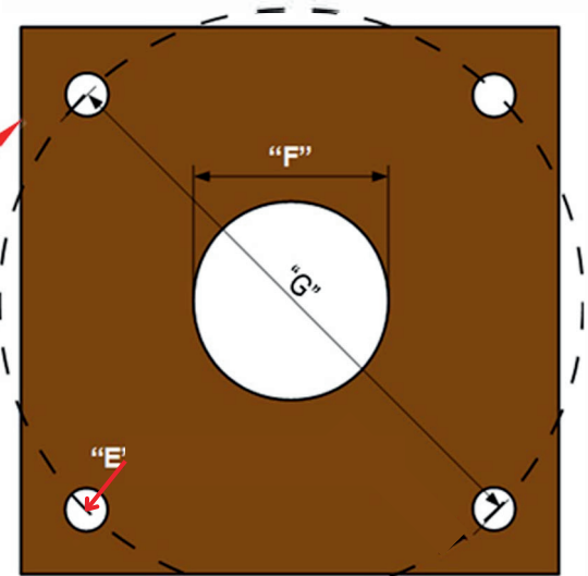
Top view of Anchor Assembly
